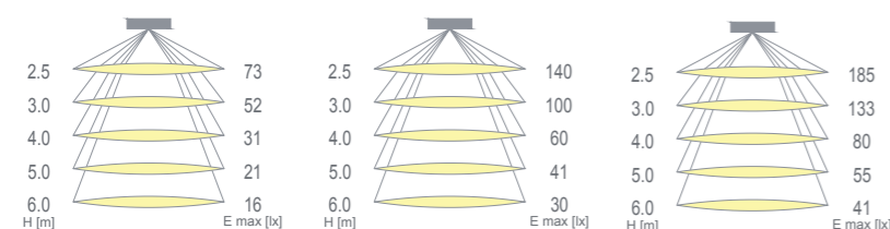
Wars LED DeLuxe 60 Standard Wars LED DeLuxe 120 Standard Wars LED DeLuxe 150 Standard
