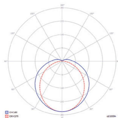
Wars LED DeLuxe 60 Standard
