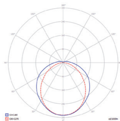
Wars LED DeLuxe 120 Standard
